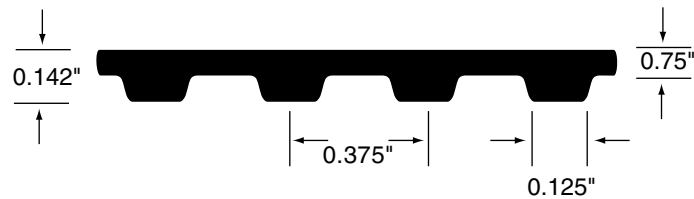
Nominal Dimensions
