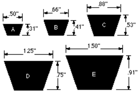
Nominal Dimensions
