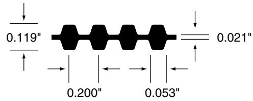
Nominal Dimensions
