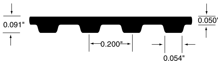
Nominal Dimensions
