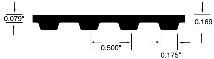
Nominal Dimensions
