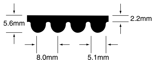
Nominal Dimensions
