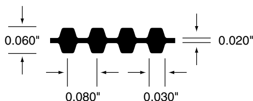
Nominal Dimensions
