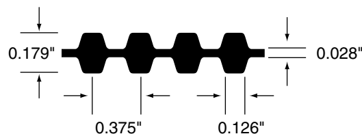
Nominal Dimensions
