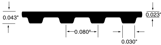
Nominal Dimensions
