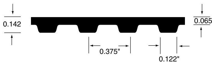
Nominal Dimensions
