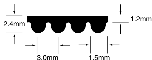
Nominal Dimensions
