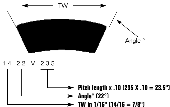
Nominal Dimensions
