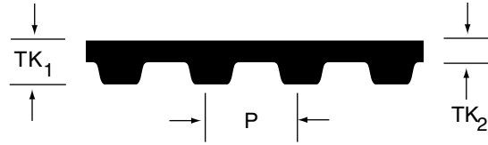
Nominal Dimensions
