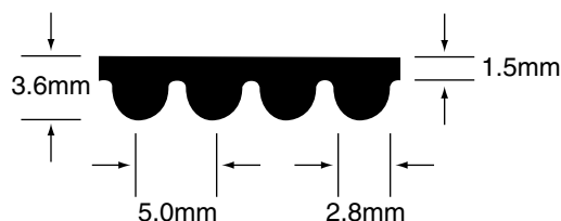
Nominal Dimensions
