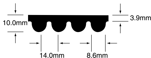
Nominal Dimensions
