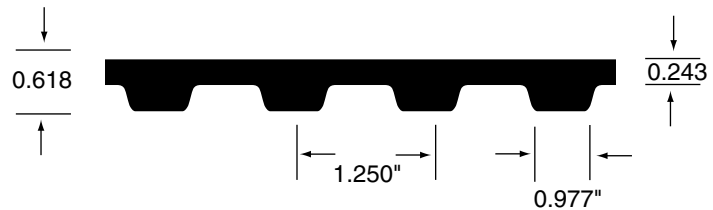
Nominal Dimensions
