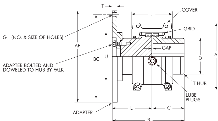
DIMENSIONS — INCHES
