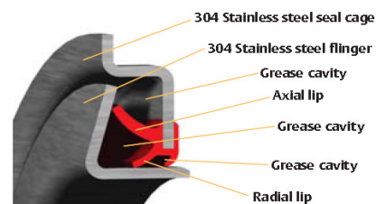
Sealmaster HPS Seal (U.S. Patent Number 6,817,769)
